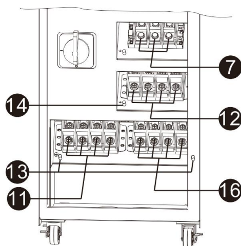
Diagram 6: 40K Input/Output Terminal
